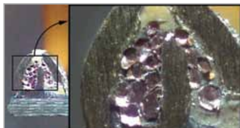
Figure 5: Cross Section of Terminated Wire
