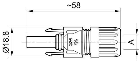
Female cable coupler PV-KBT4...
