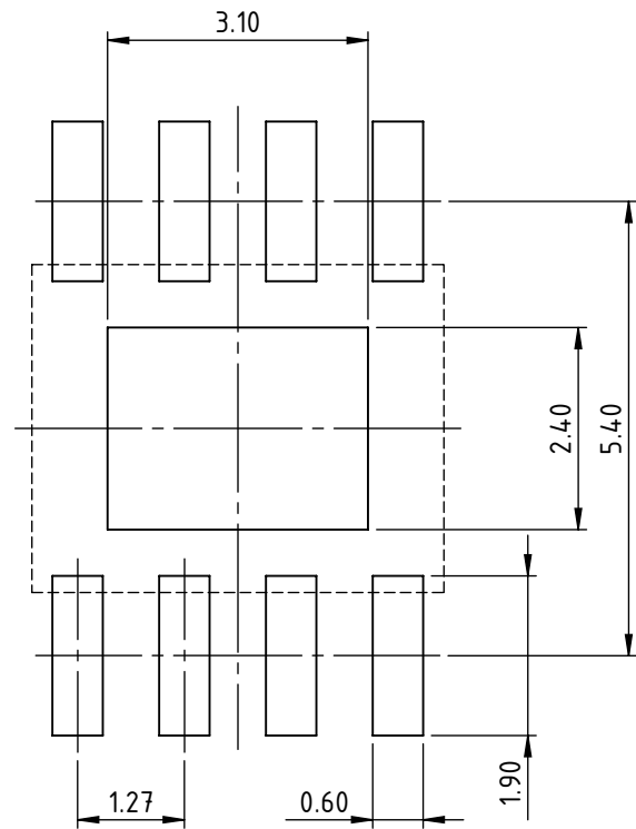
RECOMMENDED PCB-FOOTPRINT
